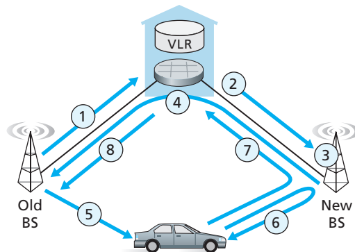
Figure 7.32 ♦ Steps in accomplishing a handoff between base stations with a common MSC
