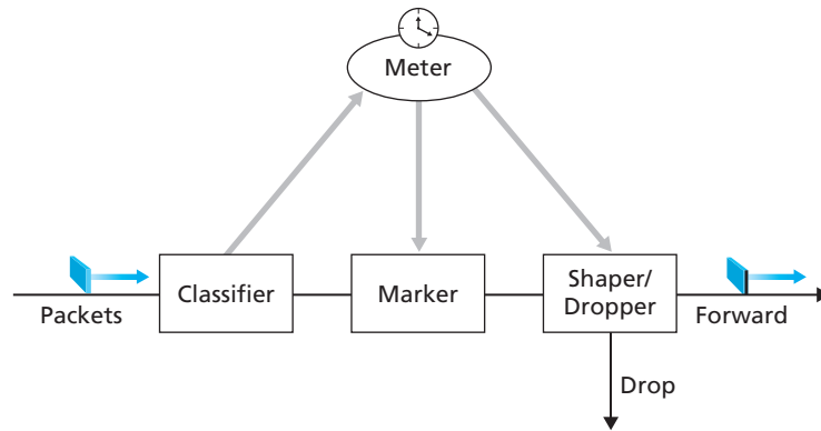
Figure 9.17 ♦ A simple Diffserv network example
