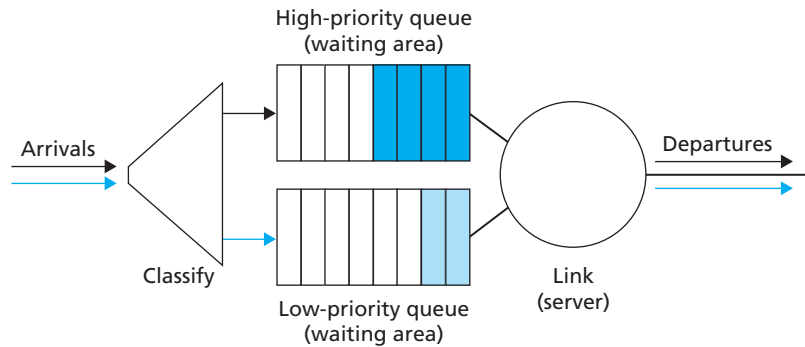
Figure 4.12 ♦ The priority queuing model
