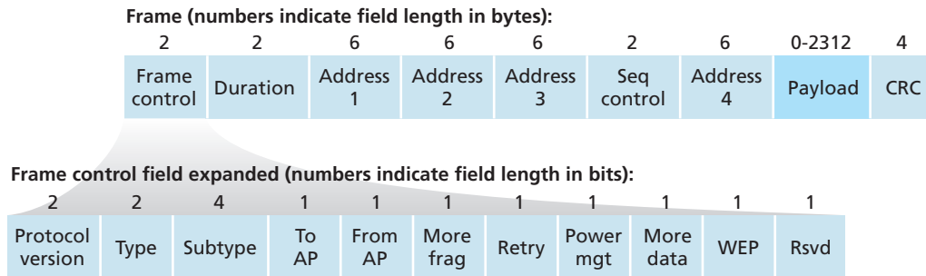
Figure 7.13 ♦ The 802.11 frame
