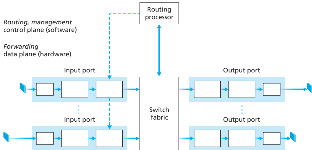
Figure 4.4 ♦ Router architecture
