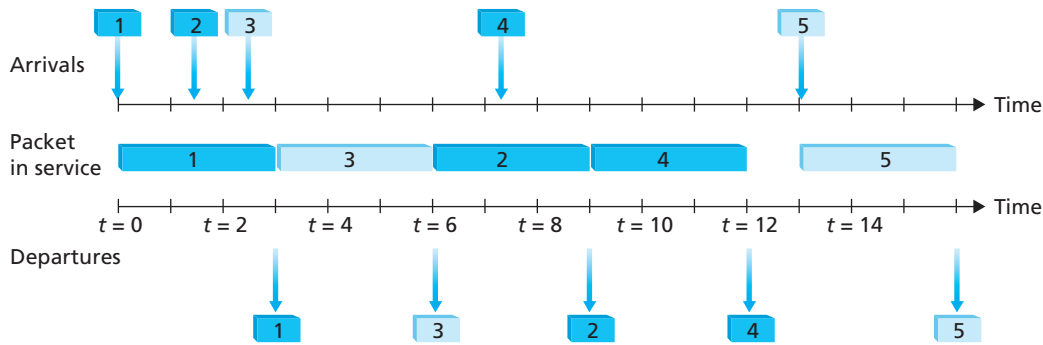
Figure 4.14 ♦ The two-class robin queue in operation
