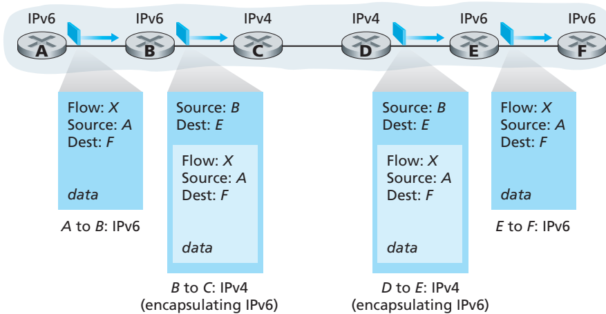
Figure 4.27 ♦ Tunneling
