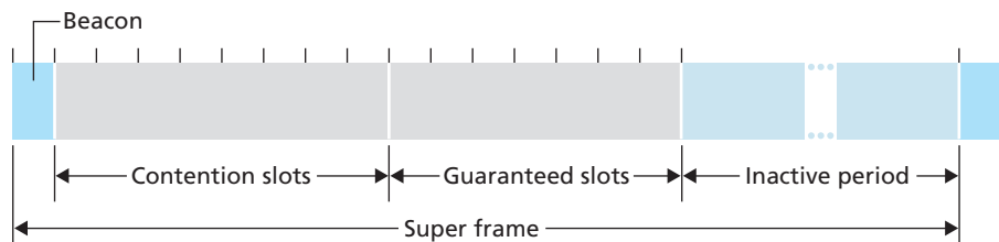
Figure 7.17 ♦ Zigbee 802.15.4 super-frame structure
