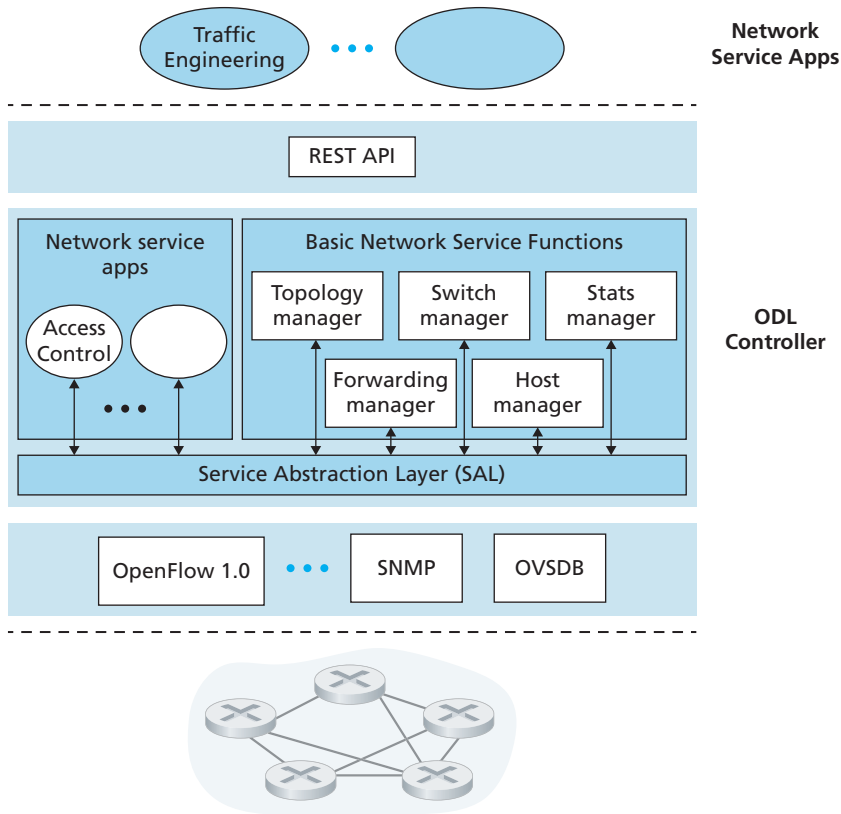
Figure 5.17 ♦ The OpenDaylight controller
