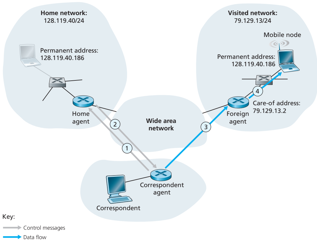
Figure 7.26 ♦ Direct routing to a mobile user
