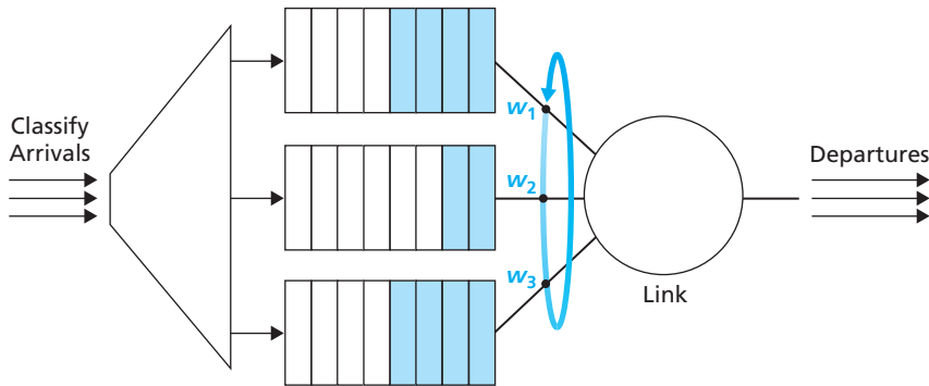
Figure 4.15 ♦ Weighted fair queuing
