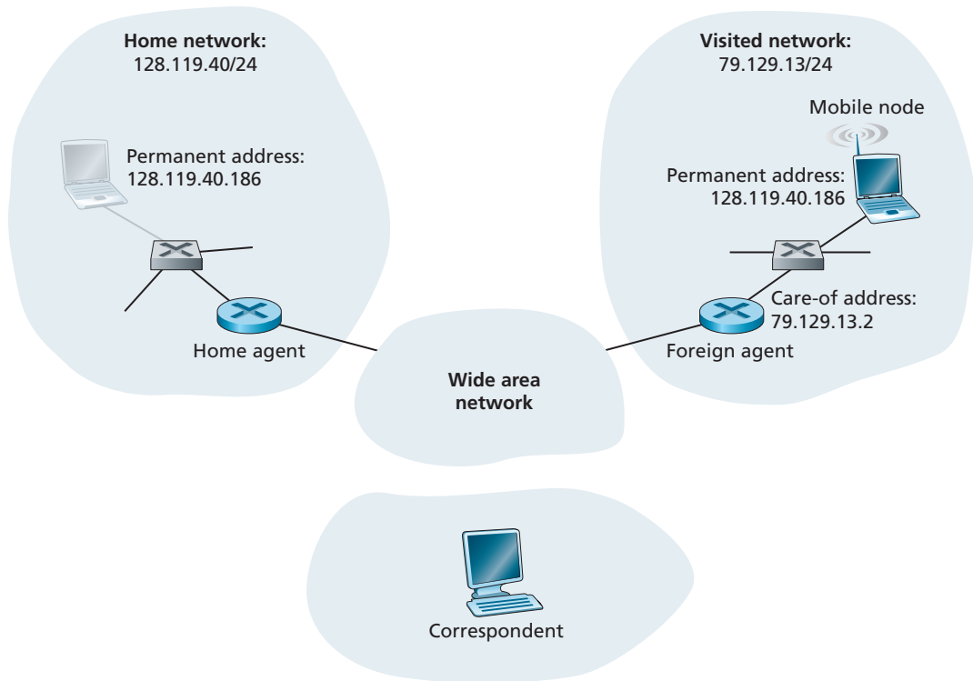
Figure 7.23 ♦ Initial elements of a mobile network architecture
