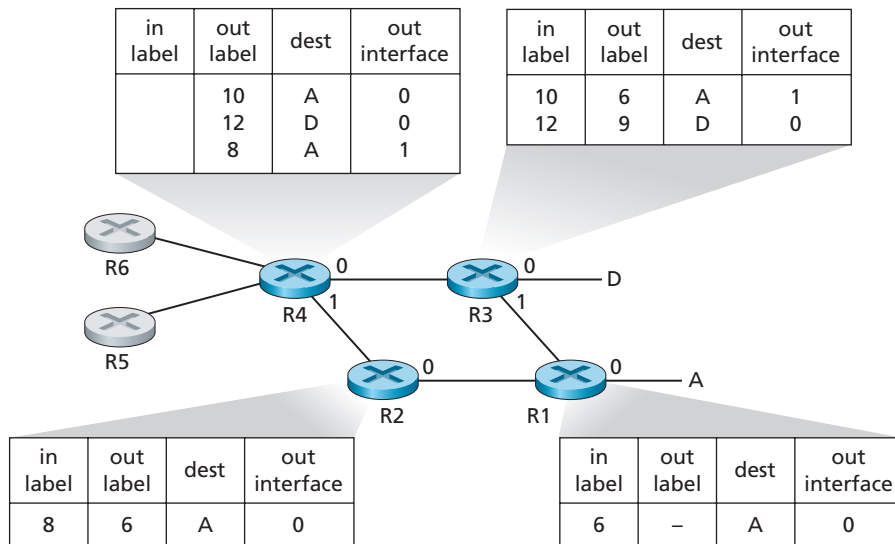
Figure 6.29 ♦ MPLS-enhanced forwarding
