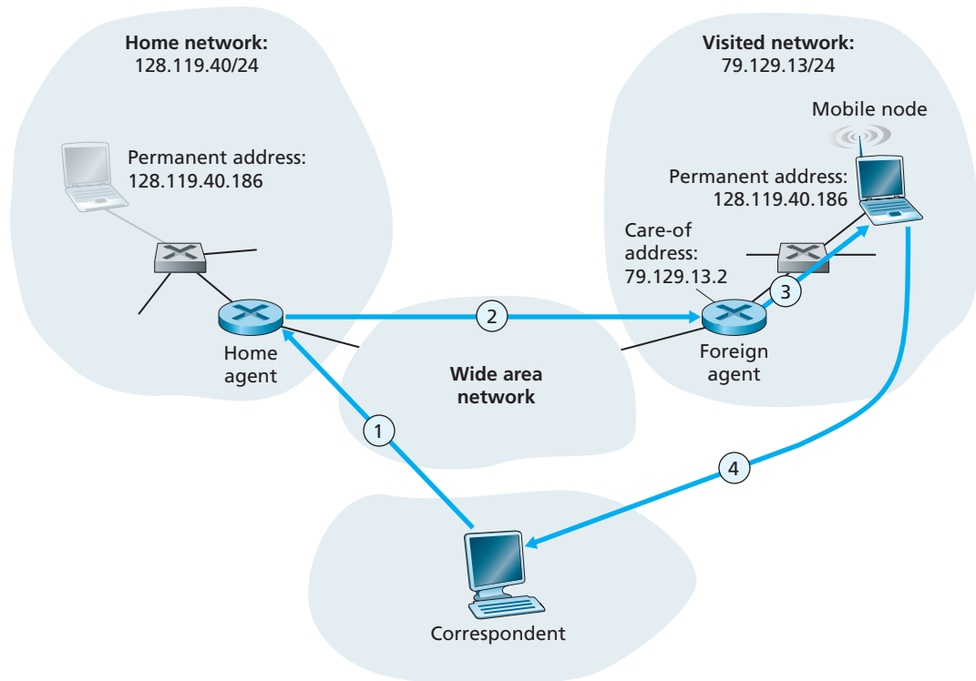
Figure 7.24 ♦ Indirect routing to a mobile node
