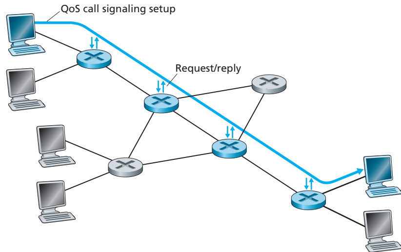
Figure 9.19 ♦ The call setup process
