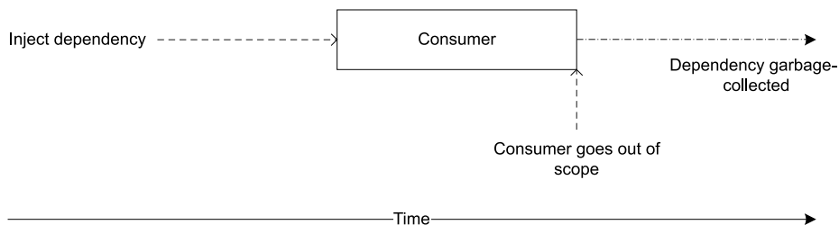
Figure 8.3 Whoever injects the DEPENDENCY into a consumer decides when it's created, but the consumer can keep the DEPENDENCY alive by holding a reference to it. When the consumer goes out of scope, the DEPENDENCY may be eligible for garbage collection.
