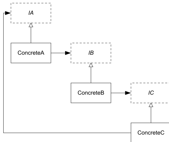
Figure 6.7 Cycles in the dependency graph can occur even if the ABSTRACTIONS have no relations to each other. In this example, each implementation implements a separate interface but also requires a DEPENDENCY. Because ConcreteC requires IA, but the only implementation of IA is ConcreteA with its DEPENDENCY on IB and so forth, we have a cycle that can't be resolved as is.
