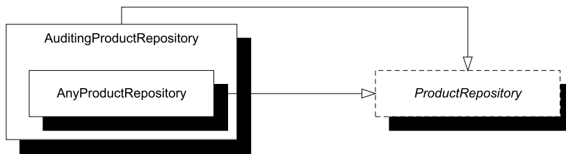
Figure 9.3 The AuditingProductRepository derives from the abstract ProductRepository class and wraps an instance of any other ProductRepository implementation. It delegates all work to the decorated ProductRepository , but adds auditing in appropriate places. Can you spot the breaching?
