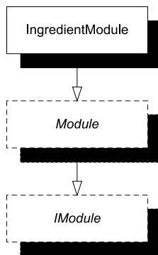
Figure 13.4 Reusable configurations can be packaged into IModule implementations. The easiest way to implement IModule is to derive from the abstract Module class—just as the IngredientModule does.
