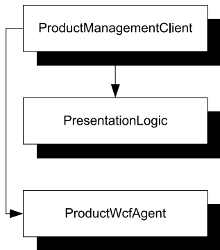
Figure 7.11 The application consists of three distinct assemblies. The ProductManagementClient assembly is the executable and contains the UI implemented in XAML with no code-behind. The PresentationLogic library contains the ViewModels and supporting classes, and the ProductWcfAgent library contains an Adapter between the custom IProductManagementAgent ABSTRACTION and the concrete WCF proxy that is used to communicate with the product-management web service. The dependency arrows imply that ProductManagementClient acts as the COMPOSITION ROOT, because it wires together the other modules.
