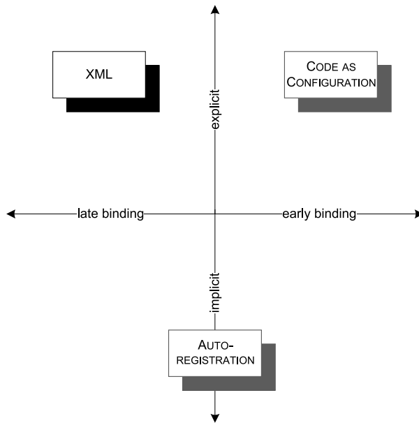
Figure 12.3 Spring.NET mainly supports XML configuration out of the three possible options outlined in chapter 3. CODE AS CONFIGURATION is only marginally supported and AUTO-REGISTRATION isn't available at all, so these options are shown in grey.
