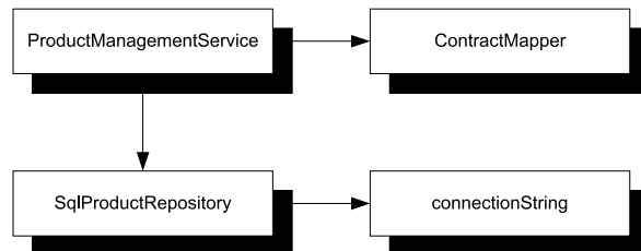
Figure 8.5 Object graph as created by CommerceServiceContainer . Each ProductManagementService instance created contains its own ContractMapper and its own SqlProductRepository , which in turn contains its own connection string. The DEPENDENCIES on the right are immutable.
