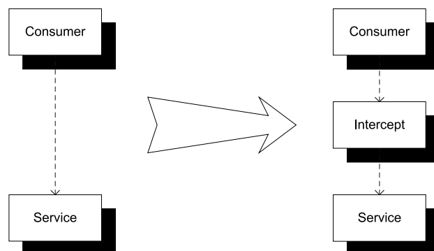
Figure 9.2 INTERCEPTION in a nutshell. We can convert a simple call from consumer to service to a more complex interaction by slotting in a piece of intermediate code. It receives the original call and passes it on to the actual implementation, while also acting on the call by doing whatever it needs to do.
