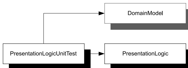
Figure 6.16 The PresentationLogicUnitTest library is a test suite that targets the PresentationLogic library. To do that, it needs a reference to its target as well as the shared ABSTRACTIONS that are defined in the Domain Model . Because PresentationLogicUnitTest doesn't target the Domain Model , the DomainModel module is shown in gray.
