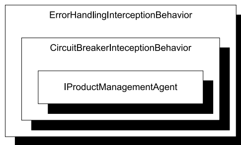
Figure 14.9 The IProductManagementAgent should be decorated by the Circuit Breaker interceptor so that when an exception is thrown by the agent, the circuit's opened for a while. The Circuit Breaker only registers exceptions but doesn't handle them, so this is the responsibility of the error handling interceptor which must be outermost to be able to handle exceptions from both the agent as well as the Circuit Breaker .
