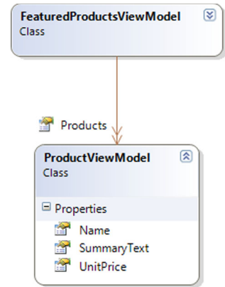
Figure 2.14 The FeaturedProductsViewModel contains a list of ProductViewModel s. Both are POCO's, which makes them eminently susceptible to unit testing. The SummaryText property is derived from the Name and UnitPrice properties to encapsulate rendering logic.
