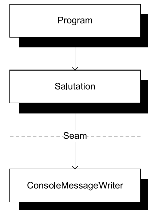
Figure 1.12 The Hello DI application from section 1.2 contains a SEAM between the Salutation and ConsoleMessageWriter classes because the Salutation class only writes through the ABSTRACTION of the IMessageWriter interface.
