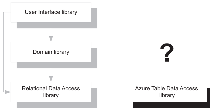
Figure 2.12 Attempting to remove the relational Data Access library leaves nothing left, because all other modules depend on it. There's no place where we can instruct the Domain library to use the new Azure Table Data Access library instead of the original.
