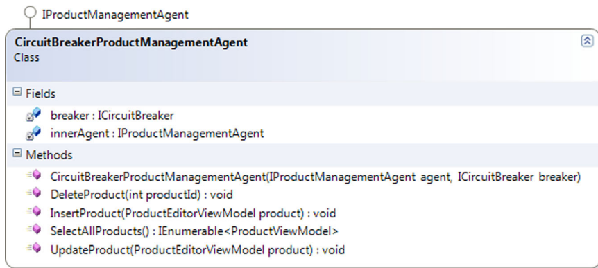
Figure 9.5 The CircuitBreakerProductManagementAgent is a Decorator of IProductManagementAgent : notice how it implements the interface and also contains an instance injected through the constructor. The other DEPENDENCY is an ICircuitBreaker that we can use to implement the Circuit Breaker pattern.
