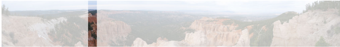
Late binding
