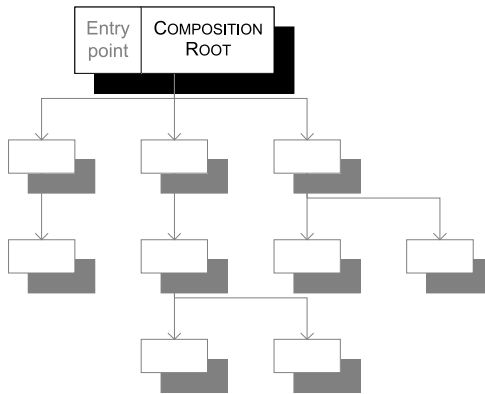
Figure 3.6 When composing an application from many loosely coupled classes, the composition should take place as close to the application's entry point as possible. The COMPOSITION ROOT composes the object graph, which subsequently performs the actual work of the application.
