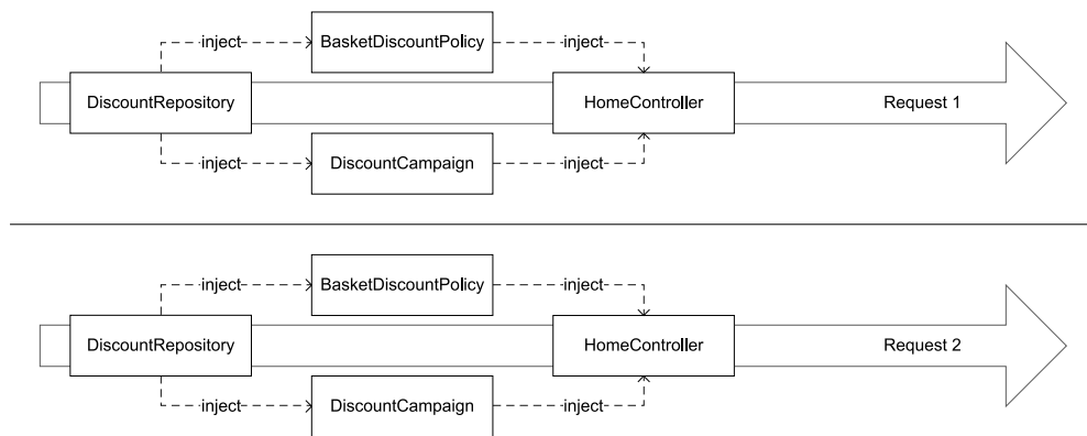
Figure 8.11 The WEB REQUEST CONTEXT lifestyle indicates that we create at most one instance per web request . The DiscountRepository instance is shared between BasketDiscountPolicy and DiscountCampaign , but only within Request 1 . Request 2 uses the same configuration, but instances are constrained to that request.
