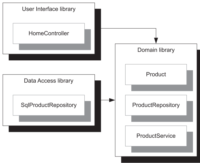
Figure 2.21 Dependency graph showing the example commerce application when Dependency Injection is applied. The most notable difference is that the Domain library no longer has any dependencies. The grey boxes within the black boxes show sample classes in each library to give you an idea which classes go where. There are more classes in each library than the ones shown.
