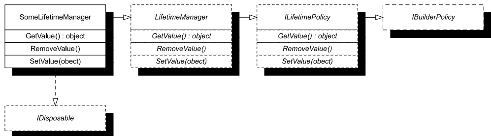
Figure 14.5 The SomeLifetimeManager implements a custom lifetime by deriving from the abstract LifetimeManager class which itself implements the ILifetimePolicy interface that derives from the IBuilderPolicy marker interface. A custom lifetime can optionally implement IDisposable to implement cleanup functionality when a container is being disposed of.
