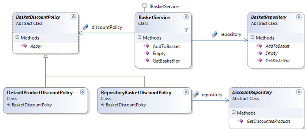
Figure 2.25 BasketService and supporting classes. A BasketService can retrieve and evaluate a Basket for a given user. It uses a BasketRepository to retrieve the Basket and a BasketDiscountPolicy to apply discounts (if any).
