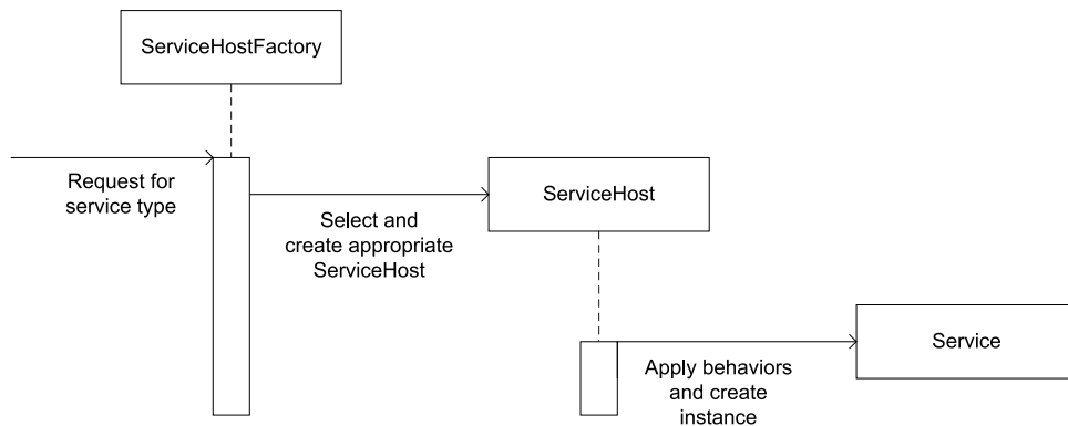
Figure 7.7 When a message (request) arrives for a service operation, WCF determines which CLR type implements the service. It asks a ServiceHostFactory to create an appropriate ServiceHost that can host the requested service. The ServiceHost does its part by applying behaviors and creating the requested instance.
