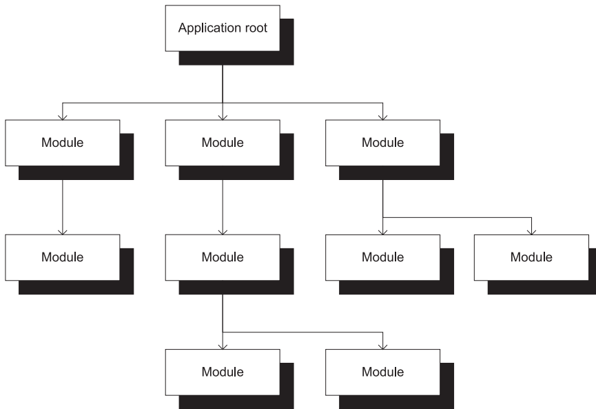
Figure 3.7 The entry point of an application is the root of a modular application. Either directly or indirectly, the root consumes the other modules. A COMPOSITION ROOT should be placed in the application's root—as close to the entry point as possible.
