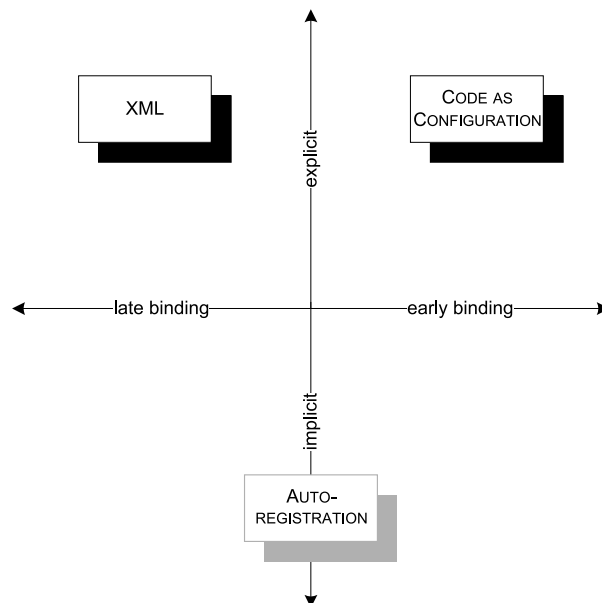
Figure 14.3 Conceptually different configuration options. CODE AS CONFIGURATION is strongly typed and tends to be explicit. XML, on the other hand, is late bound, but still explicit. AUTO-REGISTRATION instead relies on conventions that can be both strongly typed and more loosely defined, but Unity has no built-in support for that.
