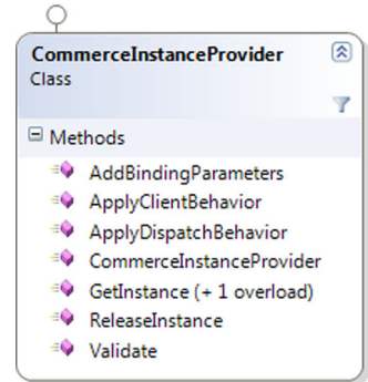
Figure 7.9 CommerceInstanceProvider implements both IInstanceProvider and IContractBehavior , so you're required to implement seven methods. You can leave three empty, and the other four are one-liners.
