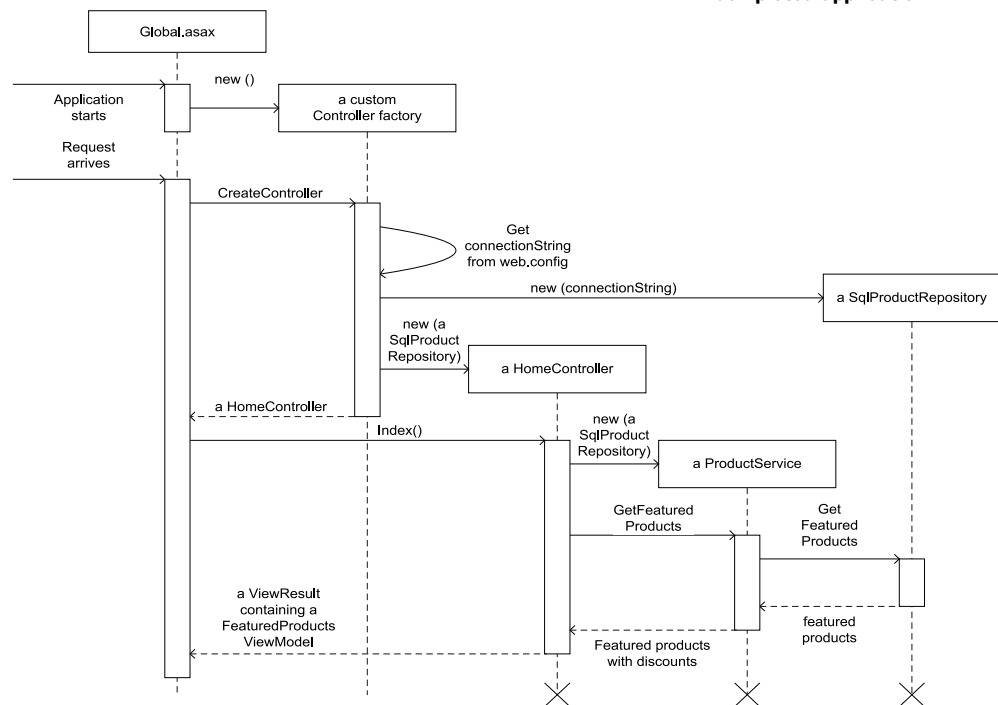
Figure 2.20 Interaction between elements involved in Dependency Injection in the Commerce application. Notice how the SqlProductRepository instance is injected into the HomeController , and then again later, through the HomeController into a ProductService that ultimately uses it.
