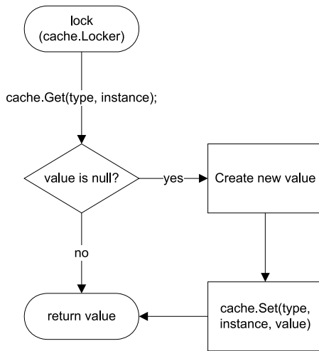
Figure 11.5 StructureMap interacts with the IObjectCache interface by first invoking the Get method on a cache object. If the cache returns a value, this value is used immediately. If not, StructureMap creates the new value and adds it to the cache before returning it.
