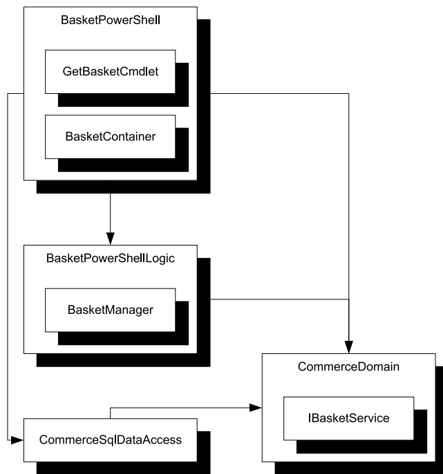
Figure 7.18 The BasketPowerShell library only contains the infrastructure necessary to make PowerShell happy—it's a HUMBLE OBJECT. As soon as the static BasketContainer has resolved a BasketManager, all further implementation happens in different assemblies. The BasketManager class has no access to the internal BasketContainer but consumes an IBasketService from the Domain Model. As usual, arrows denote references. Not all involved classes are shown.
