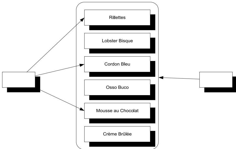
Figure 11.6 In the situation on the left, we wish to explicitly select only certain DEPENDENCIES from the larger list of all configured instances. This is different from the situation to the right, where we indiscriminately want them all.
