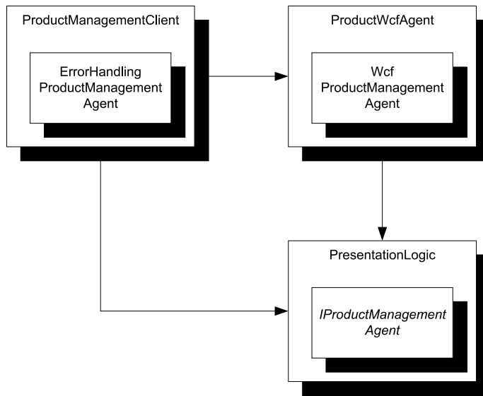
Figure 9.9 ErrorHandlingProductManagementAgent and WcfProductManagementAgent both implement IProductManagementAgent , but are defined in two different libraries. Because the ProductManagementClient assembly contains the COMPOSITION ROOT, it has a DEPENDENCY on ProductWcfAgent and PresentationLogic .
