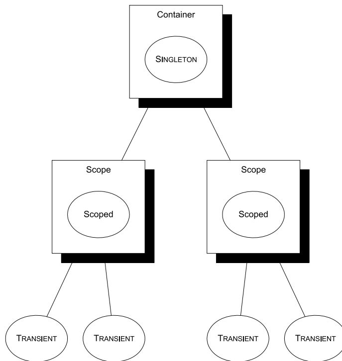
Figure 13.5 Autofac lifetime scopes act as containers that can share components for a limited duration or purpose. A lifetime scoped component is a SINGLETON within that scope. No matter how many times we ask a scope for such a component, we get the same instance. Another scope will have its own instance, and the parent container manages the truly shared SINGLETONS. TRANSIENT components are never shared, but will be decommissioned when the scope is disposed of.
