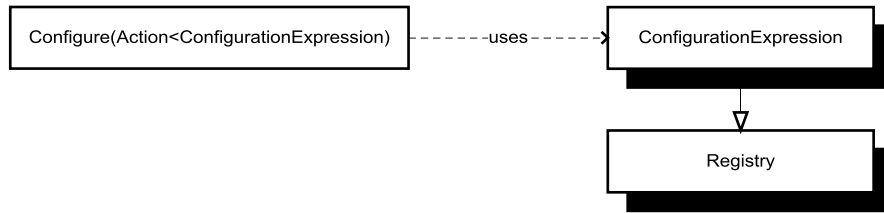
Figure 11.4 The Configure method of the Container class takes as input a delegate that operates on a ConfigurationExpression —in this chapter, we represent this ConfigurationExpression instance with the variable name x . The ConfigurationExpression class is a child class of the concrete Registry class.
