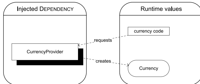
Figure 6.2 The injected CurrencyProvider is used to map a primitive runtime value (the currency code string) to a runtime DEPENDENCY (the Currency instance).
