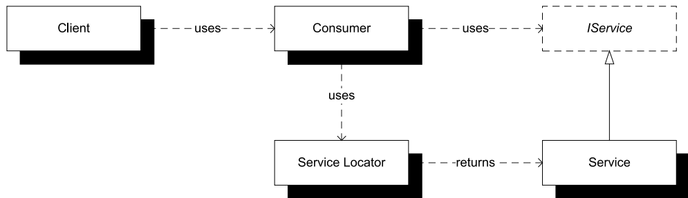
Figure 5.7 A SERVICE LOCATOR's prime responsibility is to serve instances of services when consumers request them. The Consumer uses the IService interface and requests an instance from the SERVICE LOCATOR, which then returns an instance of whatever concrete implementation it's configured to return.
