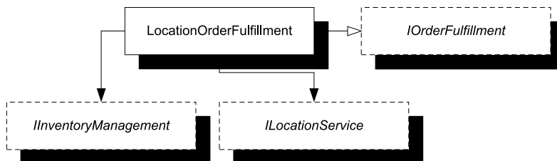
Figure 6.13 The interaction between IInventoryManagement and ILocationService is implemented in the LocationOrderFulfillment class, which implements the IOrderFulfillment interface. Consumers of the IOrderFulfillment interface have no idea that the implementation has two DEPENDENCIES .
