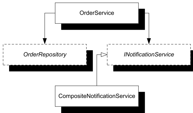
Figure 6.15 The final OrderService with refactored DEPENDENCIES . You keep OrderRepository as a separate DEPENDENCY because you need its additional methods to implement other functionality of OrderService . All the other notifications are hidden behind the INotificationService interface. At runtime, you use a CompositeNotificationService that contains the remaining three notifications.
