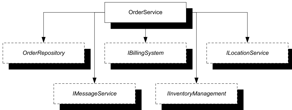
Figure 6.12 OrderService has five direct DEPENDENCIES , indicating that it violates the SINGLE RESPONSIBILITY PRINCIPLE .
