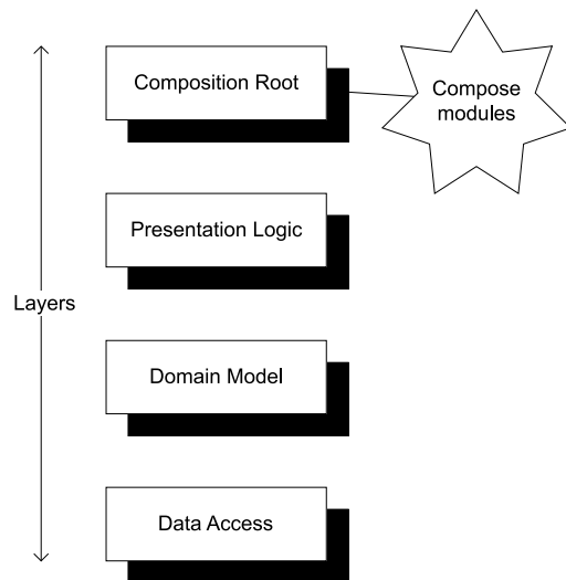
Figure 7.2 The COMPOSITION ROOT composes all the independent modules of the application. In contrast to mise en place , this doesn't happen as late as possible, but happens in a place where the integration of the different modules is required.
