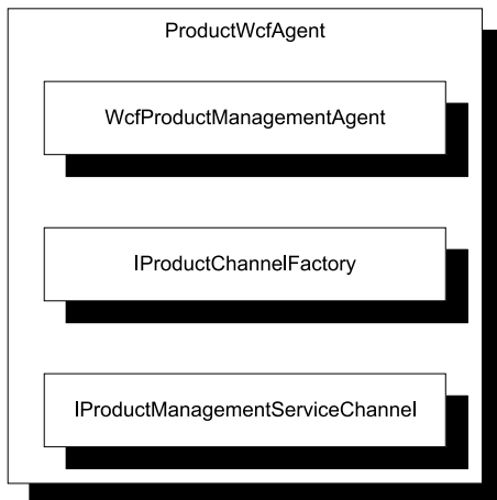
Figure 8.7 Among other types, the ProductWcfAgent library contains the implementation of IProductManagementAgent and its supporting types. WcfProductManagementAgent uses an IProductChannelFactory to create instances of IProductManagementServiceChannel , which is disposable. Although this can be considered a LEAKY ABSTRACTION, it doesn't leak very far because all consumers and implementers are contained in the same assembly.
