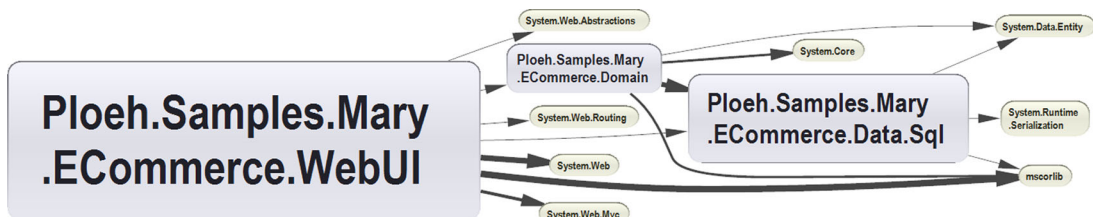
Figure 6.19 Dependency graph generated by NDepend for Mary's commerce solution. By default, NDepend includes all DEPENDENCIES, including modules from the BCL. The size of the boxes reflects the number of code lines in each module, and the thickness of the arrows reflects the number of members used across the references.
