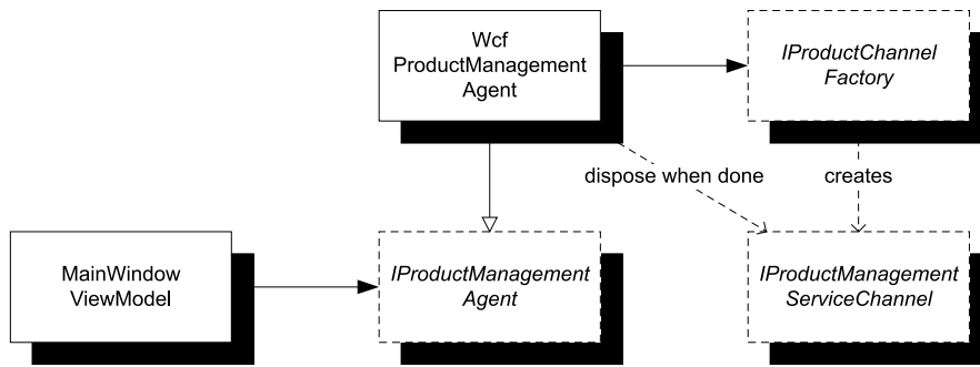
Figure 6.6 The MainWindowViewModel class consumes the IProductManagementAgent interface. This is a coarse-grained interface that exposes appropriate methods for the consumer to call. From MainWindowViewModel 's perspective, no connection management is taking place. When the application is running, the WcfProductManagementAgent class provides the implementation of the coarse-grained interface. It does this by consuming the Abstract Factory IProductChannelFactory that creates disposable instances. The IProductManagementServiceChannel interface derives from IDisposable , which enables WcfProductManagementAgent to dispose of the WCF client when the operations have been successfully invoked.
