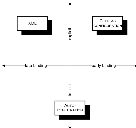
Figure 11.3 Conceptually different configuration options. CODE AS CONFIGURATION is strongly typed and tends to be explicit. XML , on the other hand, is late bound, but still explicit. AUTO-REGISTRATION instead relies on conventions that can be both strongly typed and more loosely defined.
