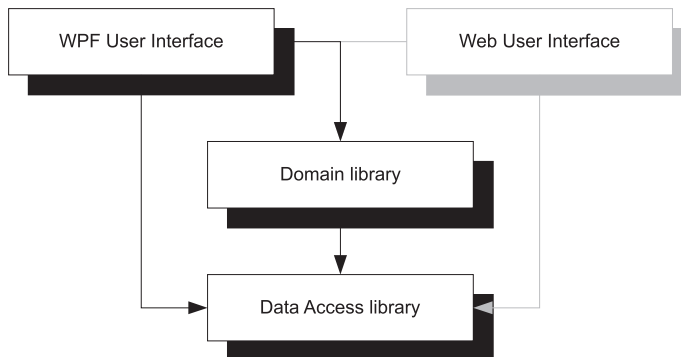
Figure 2.11 Replacing the Web User Interface with a WPF User Interface is possible because no module depends on the Web User Interface. The original Web User Interface remains in the figure in grayscale to illustrate the point that adding a new user interface doesn't preclude the original.
