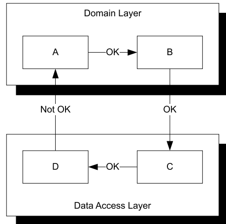
Figure 6.8 When a cycle crosses one or more layer boundaries, at least one reference is architecturally illegal. In this case, the reference from D to A is the culprit. If a situation like this occurs, it should be addressed immediately.
