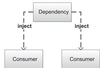
Figure 1.15 Separate consumers sharing the same type of DEPENDENCY are injected with a shared instance.
