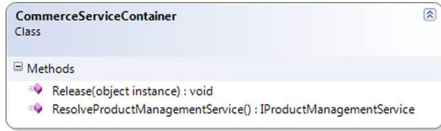
Figure 8.4 All of the CommerceServiceContainer class's implementation currently resides in the ResolveProductManagementService method. The Release method does absolutely nothing, and there are no fields or properties on the class. If you're wondering why we have the Release method, we'll get to it in section 8.2.2.
