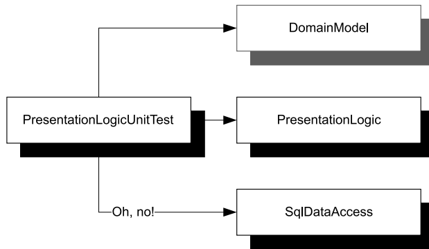
Figure 6.17 If we want type safety by adding a representative type from the SqlDataAccess library to PresentationLogicUnitTest , we introduce a new DEPENDENCY to the unit-test suite for the sole reason that we want to make sure it's never accidentally added to the PresentationLogic library. Ironic, isn't it?
