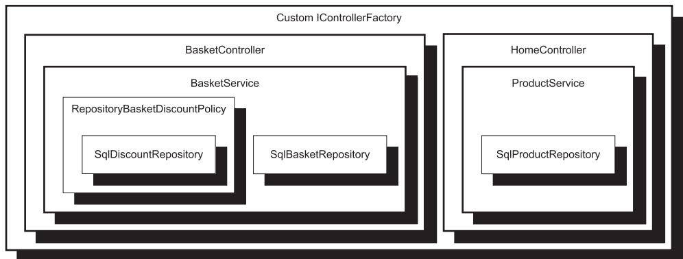
Figure 2.26 Composition of the sample commerce application with the added Basket feature, as well as the original list of featured products on the front page. Each class encapsulates its contents, and only the COMPOSITION ROOT has knowledge of all DEPENDENCIES.
