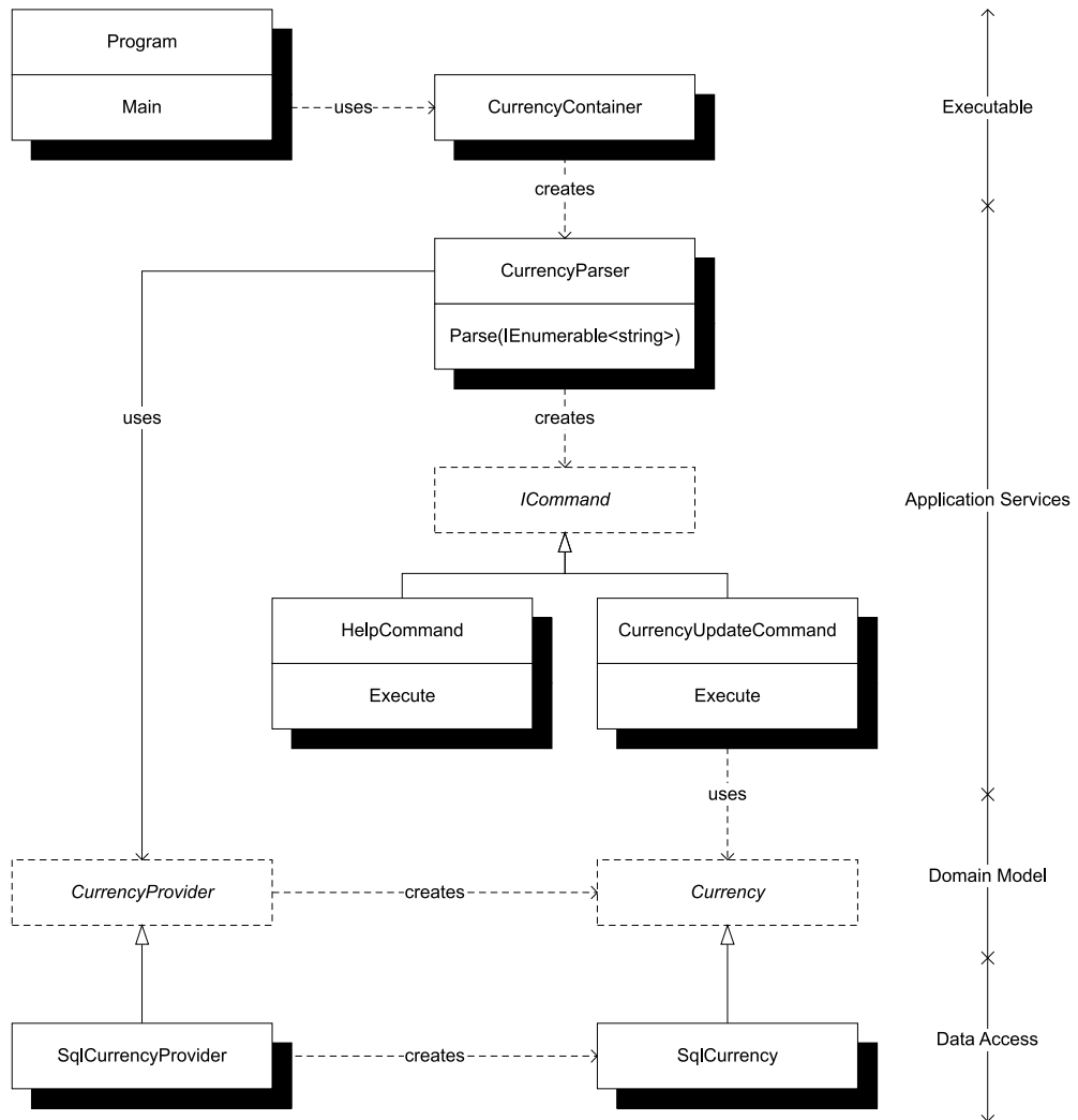
Figure 7.4 Component composition of the UpdateCurrency application. CurrencyParser parses the command-line arguments and returns an appropriate ICommand. If the arguments were intelligible, it returns a CurrencyUpdateCommand that uses a Currency instance to update the exchange rate. The vertical line to the right shows the corresponding application layer. Each layer is implemented in a separate assembly.
