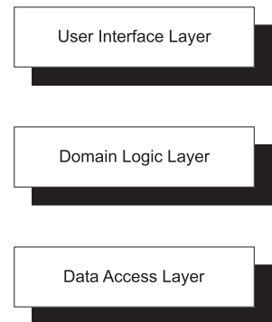
Figure 2.2 Standard three-layer application architecture. This is the simplest common variation of the n -layer application architecture, where an application is composed of n layers, each consisting of one or more modules. Some variants of n -layer diagrams will have vertical boxes that span multiple application layers. These are often used to represent Cross-Cutting Concerns , such as security or logging.
