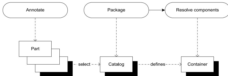
Figure 15.2 With MEF, we annotate parts (for example, classes and members) with attributes in a separate work phase. When we compose an application, we first select the appropriate parts into a catalog and then use the catalog to define a container from which we can resolve components.
