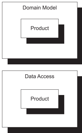
Figure 2.18 The Domain Model and Data Access libraries both define a class named Product. The Domain Product is the important class that encapsulates the Domain concept of a Product. The Data Access Product class is only an artifact of the Entity Framework wizard. It can easily be renamed or made internal.
