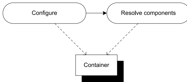
Figure 14.2 First, configure the container, and then resolve components from it. In the vast majority of cases, we create an instance of the UnityContainer class and completely configure it before we start resolving components from it. We resolve components from the same instance that we configure.
