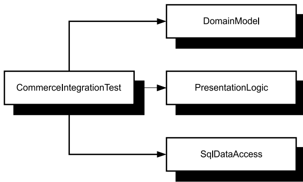
Figure 6.18 The Commerce-IntegrationTest project contains automated tests that verify that the relationships between modules are correct. Unlike unit tests, an integration-test suite can contain as many references as are necessary to perform the test.
