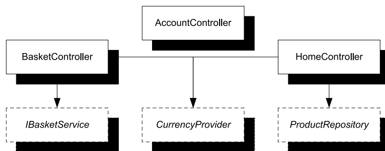
Figure 7.6 Dependency graph for the three Controllers in the sample Commerce application. The concrete implementations of each of these DEPENDENCIES have other DEPENDENCIES but these aren't shown. BasketController and HomeController share a DEPENDENCY on CurrencyProvider . AccountController is inherited unchanged from the default ASP.NET MVC template; because it uses BASTARD INJECTION, it has no unresolved DEPENDENCIES.
