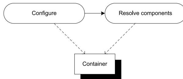
Figure 11.2 The overall usage pattern of StructureMap is simple: First we configure the container, and then we resolve components from it. In the vast majority of cases, we create an instance of the Container class and completely configure it before we start resolving components from it. We resolve components from the same instance that we configure.
