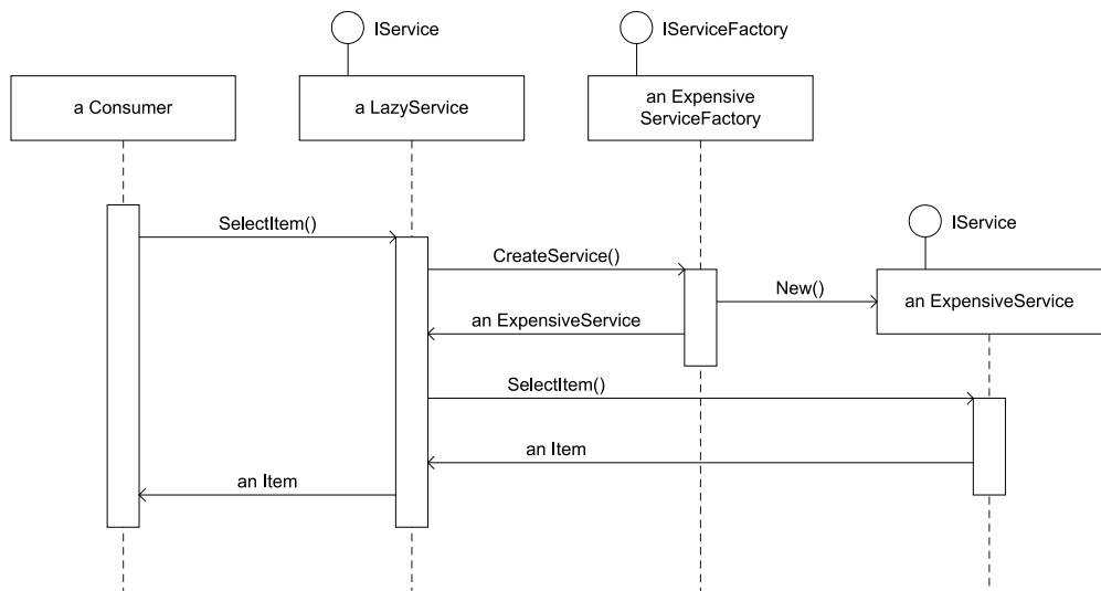
Figure 8.13 A consumer requires an IService DEPENDENCY , but if it only uses this DEPENDENCY in a small fraction of the time, it can live for a long time before requiring the services of IService . When it finally invokes IService.SelectItem() , LazyService uses its injected IServiceFactory to create an instance of another IService . It isn't until this point that the ExpensiveService instance is created. After ExpensiveService is created, all subsequent calls can be delegated to it.
