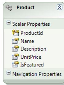
Figure 2.5 The Product entity generated from the Product database table shown in figure 2.4. Mary has changed the name of the Featured column to IsFeatured , as well as changed a few names in the generated ObjectContext (not shown).
