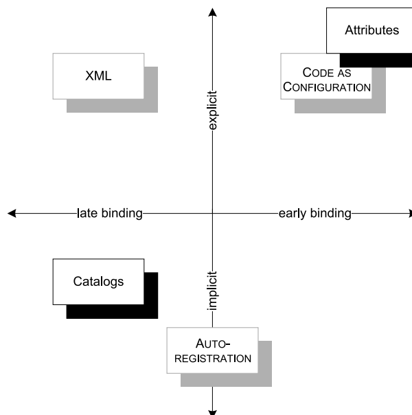
Figure 15.3 MEF doesn't fit into our standard conceptual model for configuration options, because we can't configure the container. All the normal options we're used to reviewing are unavailable and grayed out. Annotating parts with attributes defines the configuration statically together with the type, whereas catalogs provide flexibility.
