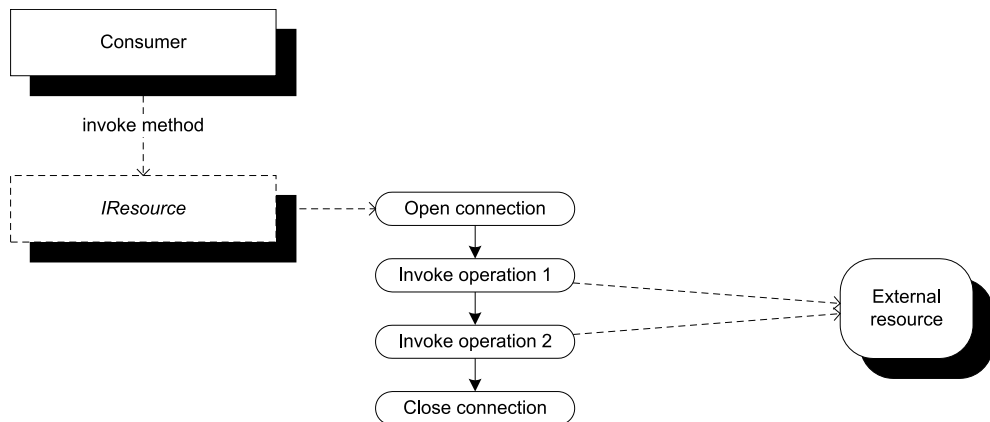
Figure 6.3 We can design an interface so that it's sufficiently coarse-grained that each method encapsulates all interactions with an external resource in a single batch. The Consumer invokes a method on the IResource interface. An implementation of that method could open a connection and invoke several methods against the external resource before closing the connection and returning a result to the consumer.
