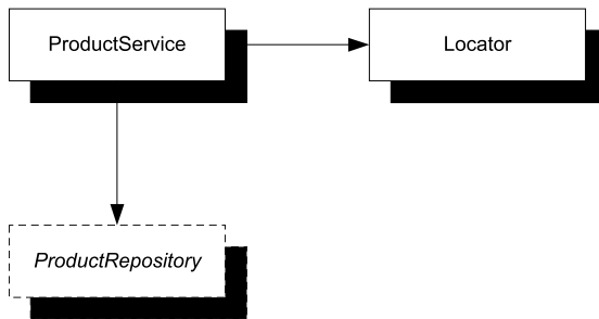
Figure 5.8 Dependency graph for a ProductService implementation that uses a SERVICE LOCATOR to serve instances of the abstract ProductRepository class
