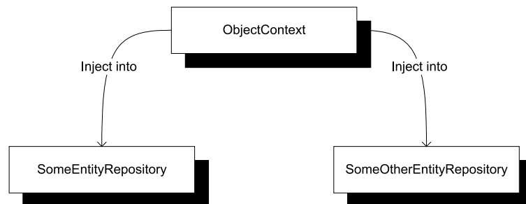
Figure 5.4 In this example, we wish to create a single instance of the ObjectContext class and inject the same instance into both Repositories . This is possible only if we can inject the instance from the outside.
