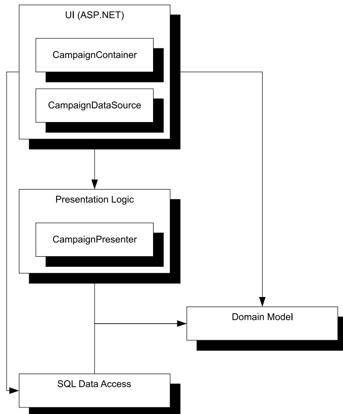
Figure 7.16 The root of the CampaignManagement application is the only part of the application that references ASP.NET. The CampaignDataSource class has a default constructor but acts as a COMPOSITION ROOT and HUMBLE OBJECT that delegates all method calls to a CampaignPresenter. As usual, the arrows denote references, and the root application references all other modules because it wires them together. Both the Presentation Logic and Data Access modules reference the Domain Model library. Not all involved classes are shown.
