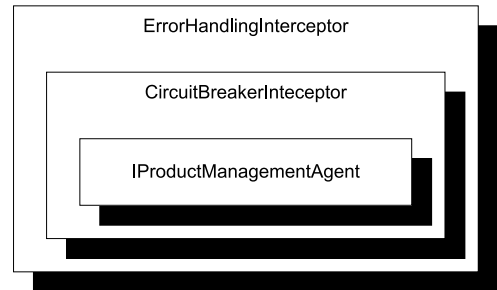
Figure 12.6 The IProductManagementAgent should be decorated by the Circuit Breaker interceptor so that when an exception is thrown by the agent, the circuit's opened for a while. Because the Circuit Breaker only registers exceptions, but doesn't handle them, this is the responsibility of the error handling interceptor, which must be outermost to be able to handle exceptions from both the agent as well as the Circuit Breaker .
