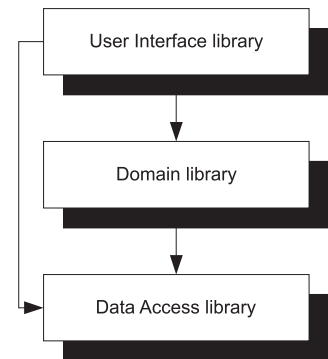
Figure 2.10 Dependency graph for Mary's application showing how the modules depend on each other. The arrows point towards a module's DEPENDENCY .
