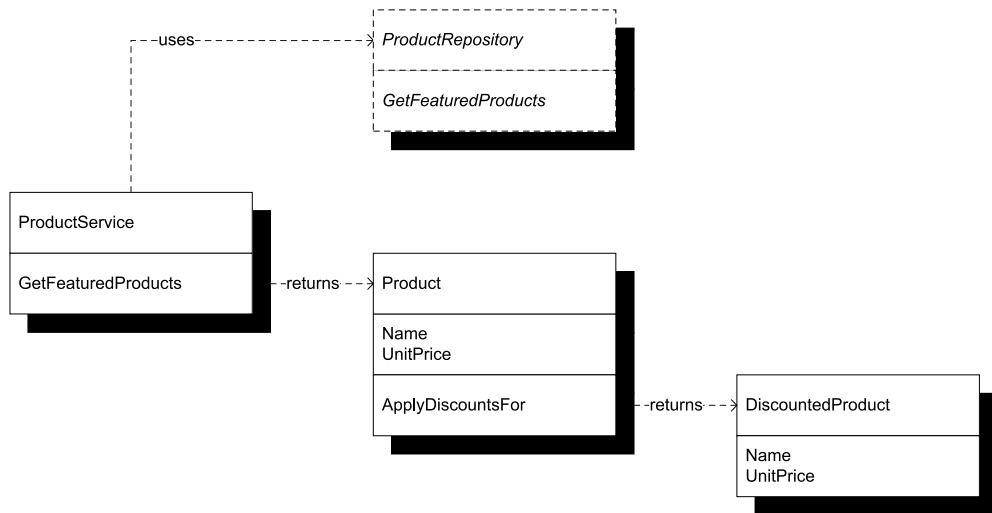
Figure 2.16 The Product class only contains the Name and UnitPrice properties, because these are the only properties needed to implement the desired application feature. The ApplyDiscountFor applies the discount (if any) for a user and returns an instance of the DiscountedProduct class. The abstract GetFeaturedProducts returns a sequence of Products .
