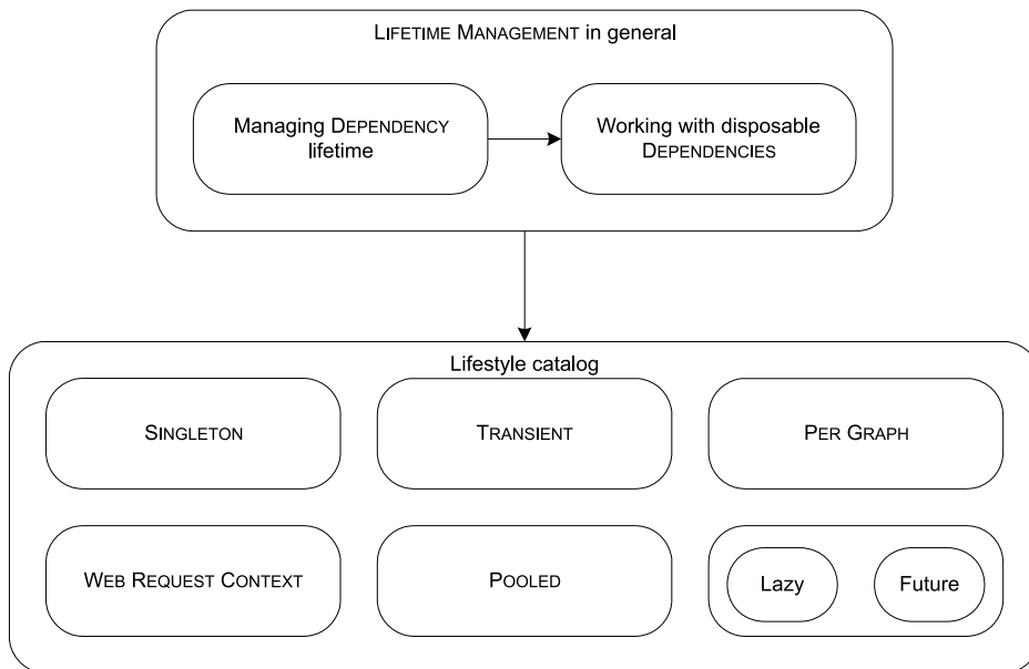
Figure 8.2 The overall structure of this chapter. We'll start with a general discussion about managing DEPENDENCY lifetime, including a particular discussion of dealing with disposable objects. We need that foundation to efficiently discuss the common patterns of the small lifestyle catalog that follows. We'll start by looking at some common and highly useful patterns and finish with a brief glance at some more exotic lifestyle scopes to give you an impression of the breadth of the topic.
