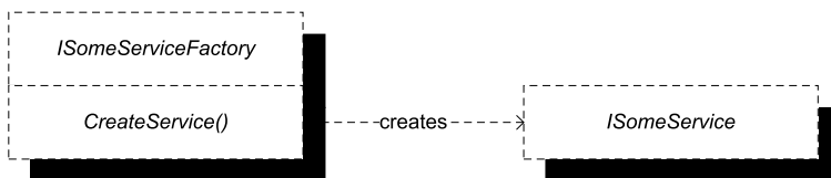
Figure 5.5 ISomeService represents the real DEPENDENCY . However, to keep its implementers free of implicit constraints, you attempt to solve the late-binding challenge by introducing the ISomeServiceFactory that will be used to create instances of ISomeService . And you will require of any factories that they have a default constructor.
