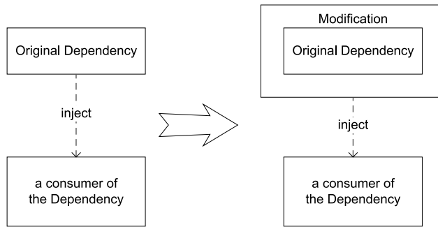
Figure 1.16 Instead of injecting the originally intended DEPENDENCY , we can modify it by wrapping another class around it before we pass it on to its consumer. The dotted arrows indicate the direction of the action—the direction of DEPENDENCY goes the opposite way.
