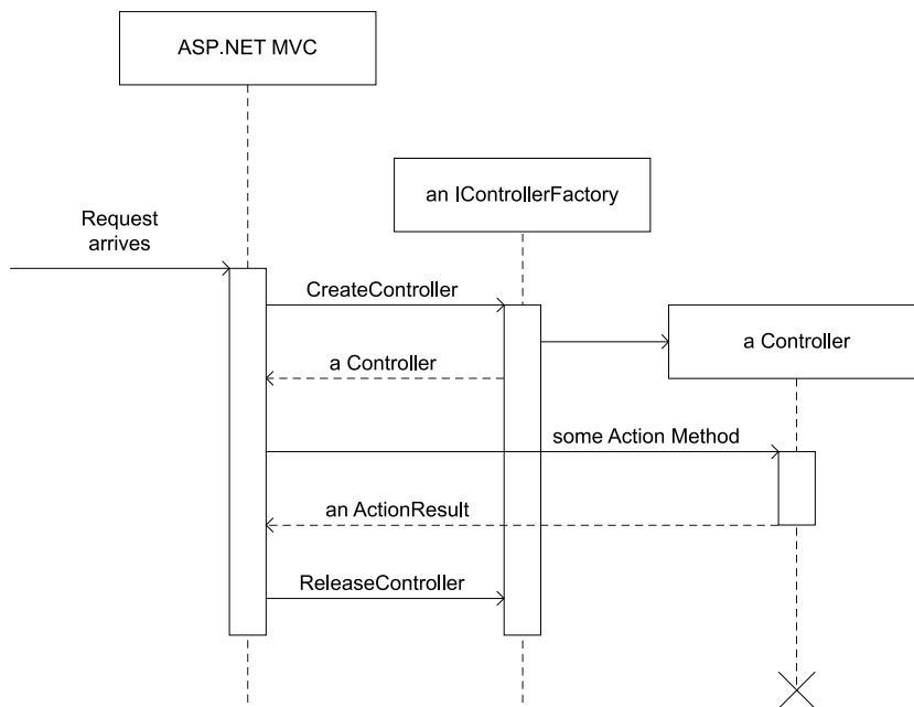
Figure 7.5 When the ASP.NET MVC runtime receives a request, it asks its Controller Factory to create a Controller for the requested URL. The Controller Factory determines the correct type of Controller to use for the given request and creates and returns a new instance of that type. ASP.NET MVC then invokes the appropriate action method on the Controller instance. When it's finished, ASP.NET MVC gives the Controller Factory a chance to dispose of resources by calling ReleaseController .
