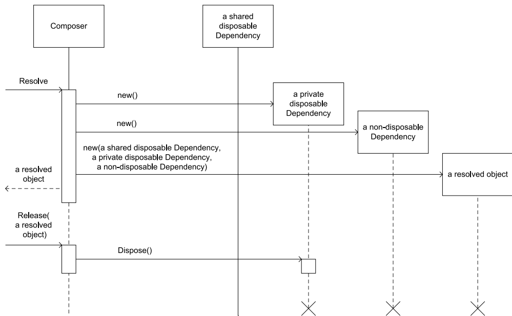
Figure 8.8 When a COMPOSER is asked to resolve an object, it gathers all of the requested object's DEPENDENCIES. In this case, the requested object has three DEPENDENCIES, and two of them are disposable. One of these disposable DEPENDENCIES is shared with other consumers, so it's reused, whereas the other DEPENDENCIES are instantiated on the spot. When the request to release the object comes in, the COMPOSER disposes of the private disposable DEPENDENCY and lets the non-disposable DEPENDENCY and the object itself go out of scope. The only interaction with the shared DEPENDENCY is that it's injected into the requested object; but because it's shared, it isn't disposed of (yet).
