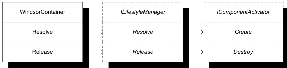
Figure 10.5 An ILifestyleManager acts as a sort of interceptor that's called instead of the underlying IComponentActivator . An ILifestyleManager implementation is expected to use the supplied IComponentActivator to create object instances. Because the ILifestyleManager sits in the middle, it gets a chance to intercept each call and perform its own lifecycle logic. It's free to reuse instances instead of calling through to the IComponentActivator each time.
