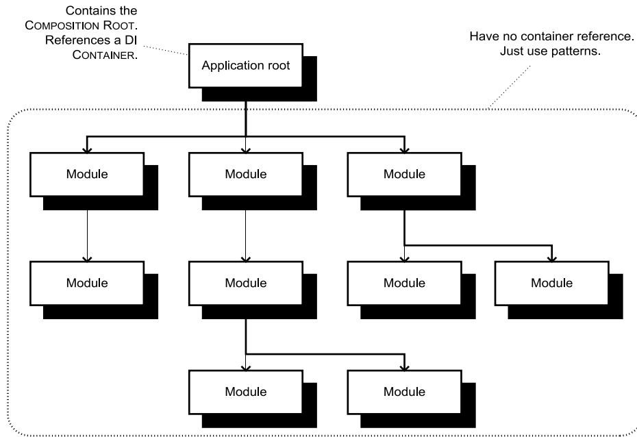
Figure 3.8 Only the COMPOSITION ROOT contained in the application root should have a reference to a DI CONTAINER. All other modules in the application should rely entirely on DI patterns and have no reference to the container.
