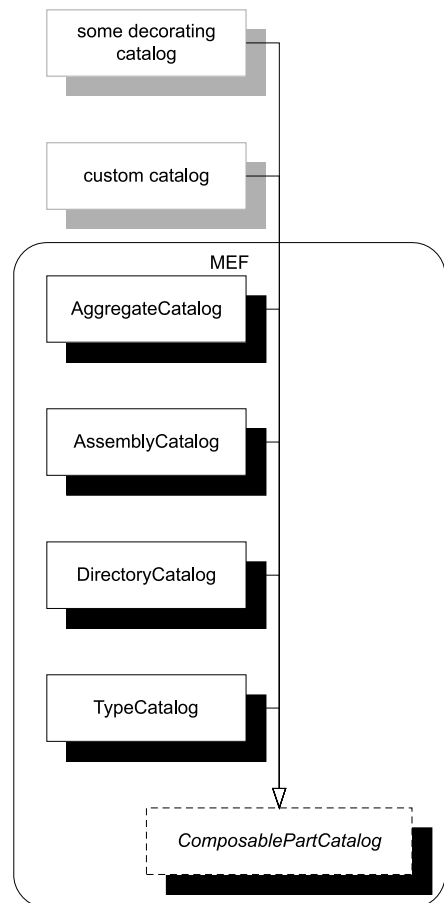
Figure 15.4 MEF include four concrete catalogs, but we can also conceivably define custom catalogs. It may be fairly straightforward to implement a catalog that acts as a Decorator for other catalogs (for example, a filtering catalog), whereas a true custom catalog would be more involved.
