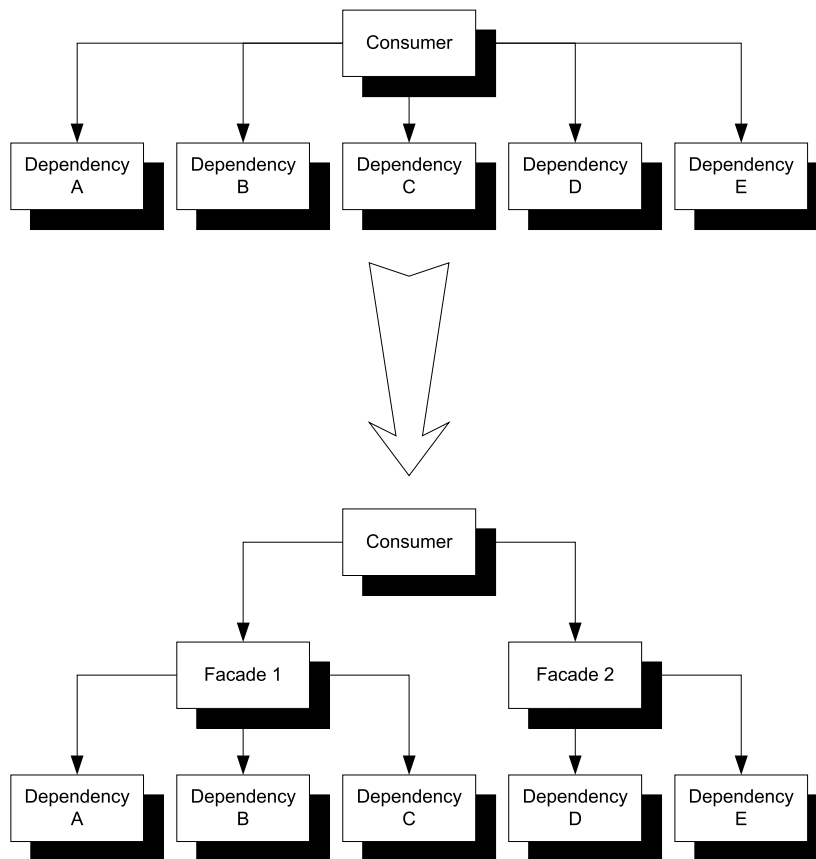
Figure 6.11 In the top diagram, the consumer has five DEPENDENCIES, which is a strong indication that it violates the SINGLE RESPONSIBILITY PRINCIPLE. Still, if the role of the consumer is to orchestrate those five DEPENDENCIES, we can't throw any away. Instead, we can introduce Facade Services that orchestrate parts of the relationship. In the bottom diagram, the consumer has only two DEPENDENCIES, and the Facades have two and three DEPENDENCIES.
