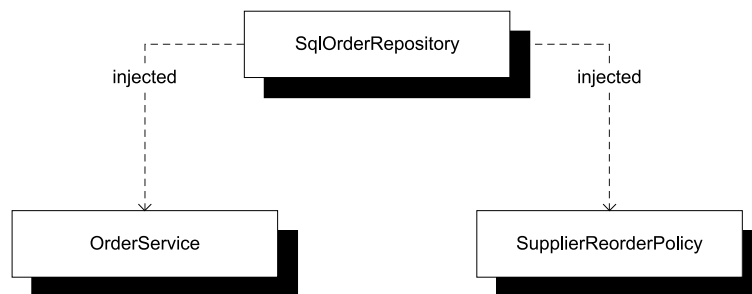
Figure 8.6 A single instance of SqlOrderRepository is injected into both OrderService and SupplierReorderPolicy . These two instances share the same DEPENDENCY. If OrderService disposes its injected OrderRepository , it destroys SupplierReorderPolicy 's DEPENDENCY, and exceptions will be thrown when SupplierReorderPolicy tries to use it.
