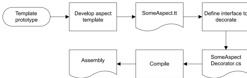
Figure 9.10 T4 makes it possible to auto-generate Decorator code from templates. The starting point is a template prototype that understands the basic concept of Decorator. The template prototype contains the code generation code that will generate the frame of the decorating class, but it doesn't define any aspect code. From the template prototype, an aspect template that describes how a specific aspect (such as Circuit Breaker) should be applied when decorating any interface is developed. The result of that is a specialized template ( SomeAspect.tt ) for that particular aspect, which can be used to generate Decorators for particular interfaces. The result is a normal code file ( SomeAspectDecorator.cs ) that compiles normally together with other code files.
