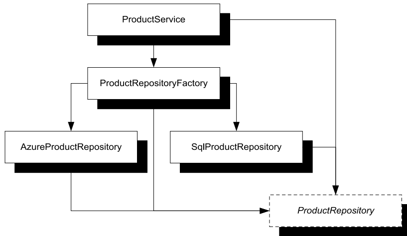
Figure 5.2 Dependency graph for the proposed solution: a static ProductRepositoryFactory is used to create ProductRepository instances
