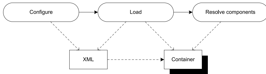
Figure 12.2 The overall usage pattern of Spring.NET involves three steps: first, we define how objects are configured and composed in an XML file. Second, we load that XML configuration into a container instance. In the third and final step, we can resolve objects from the container instance.
