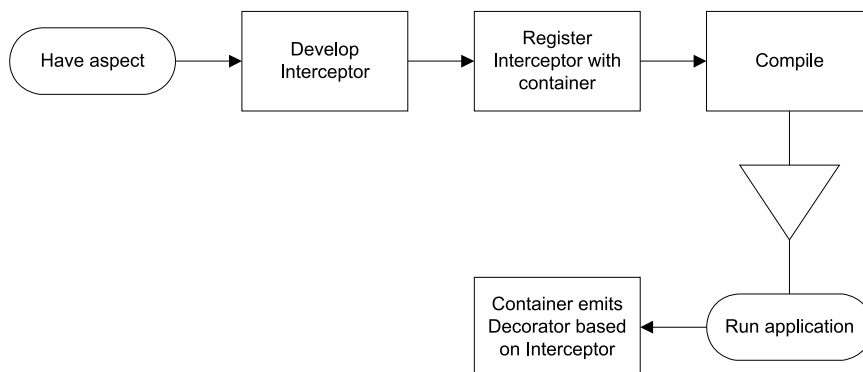
Figure 9.11 Some DI CONTAINERS allow us to define aspects as Interceptors. The Interceptor is a piece of code that implements the aspect and integrates with the container. Registering the Interceptor with the container enables the container to dynamically create and emit Decorators that contain the aspect behavior. These classes only exist at runtime.
