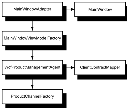
Figure 7.12 Dependency graph for MainWindowAdapter , which ends up being the root object in the application. It uses a MainWindowViewModelFactory to create the appropriate ViewModel and assign it to the MainWindow . To create MainWindowViewModel , the factory needs a WcfProductManagementAgent to pass to the ViewModel . This agent is an Adapter between IProductManagementAgent and the WCF proxy. It requires a ProductChannelFactory to create instances of the WCF proxy, as well as an IClientContractMapper that can translate between ViewModels and WCF Data Contracts.
