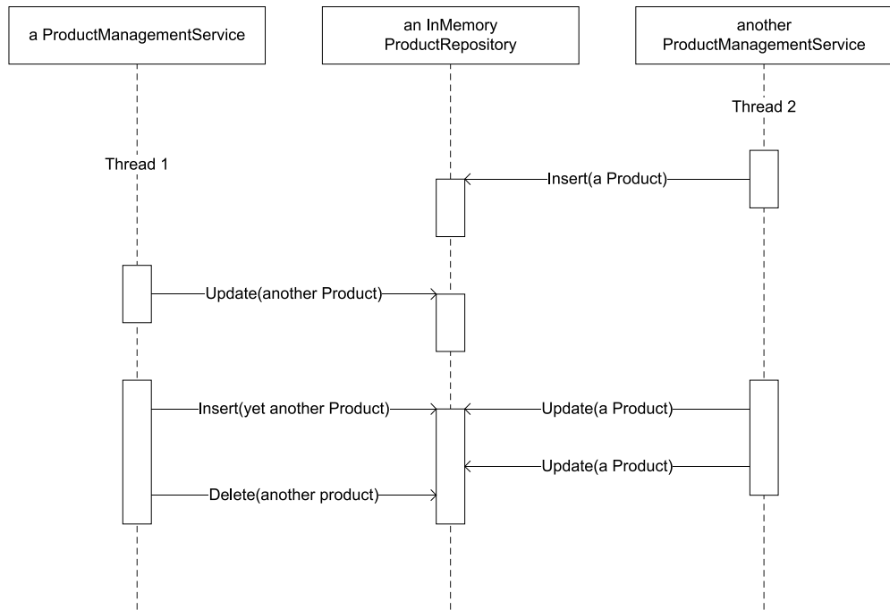
Figure 8.10 When multiple ProductManagementService instances running on separate threads access a shared resource such as an in-memory ProductRepository , we must ensure that the shared resource is thread-safe.
