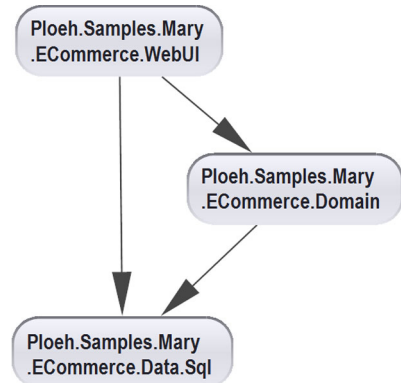
Figure 6.20 Modified NDepend graph for Mary's commerce solution. In this graph, I've manually removed all BCL modules and made the boxes and arrows the same size.
