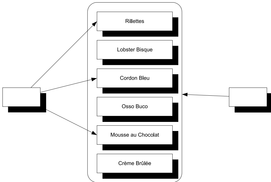
Figure 13.6 In the situation on the left, we wish to explicitly select only certain DEPENDENCIES from the larger list of all registered components. This is different from the situation on the right, where we indiscriminately want them all.
