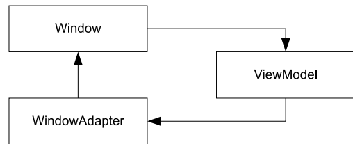
Figure 6.10 A WPF MVVM cycle. In MVVM, a Window depends on a ViewModel, which in turn depends on an IWindow instance. The proper implementation of IWindow is WindowAdapter, which depends on a WPF Window to be able to set the owner of each Window to avoid focus bugs.
