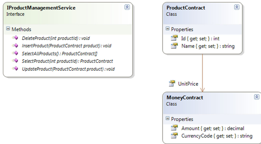
Figure 7.8 IProductManagementService is a WCF service that defines simple CRUD operations on products. It uses the associated ProductContract and MoneyContract to expose these operations. Although not shown in this diagram, all three types are decorated with the usual WCF attributes: ServiceContract , OperationContract , DataContract , and DataMember .
