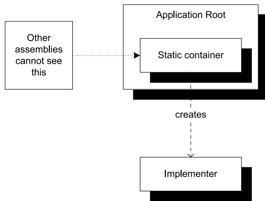
Figure 7.17 When there is no way around a static container, we can make it internal and place it in the application's root assembly. All Resolve methods return classes defined in other assemblies. Thus as soon as the container has resolved the implementer, no classes in the resolved dependency hierarchy have access to the static container because they're all outside the application's root assembly and the container is internal.
