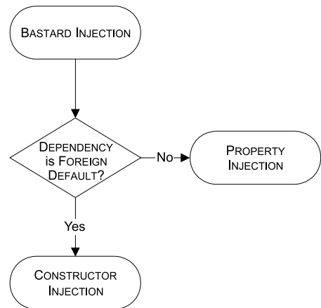
Figure 5.3 When refactoring from BASTARD INJECTION, the deciding factor is whether the DEPENDENCY is a LOCAL or FOREIGN DEFAULT.
