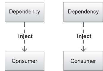
Figure 1.14 Each consumer sharing the same type of DEPENDENCY is injected with its own private instance.
