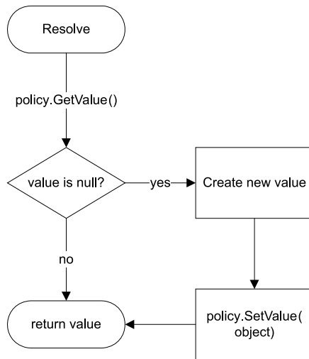
Figure 14.6 Unity interacts with the ILifetimePolicy interface by first invoking the GetValue method. If the policy returns a value, this value is used immediately. If not, Unity creates the new value and sets the value on the policy before returning it.
