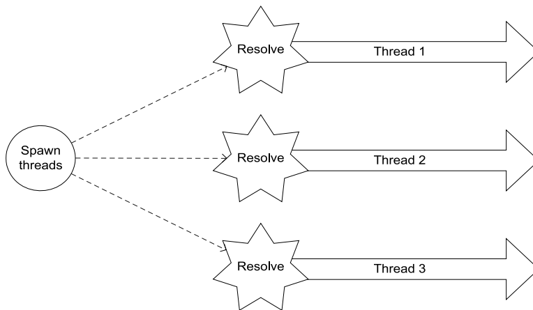
Figure 8.12 When an application immediately spins up a number of parallel tasks and resolves DEPENDENCIES from within each thread, we can use the Thread Context lifestyle to ensure that any DEPENDENCIES that aren't thread-safe can be shared among any number of consumers on the same thread. Each thread has its own instances.
